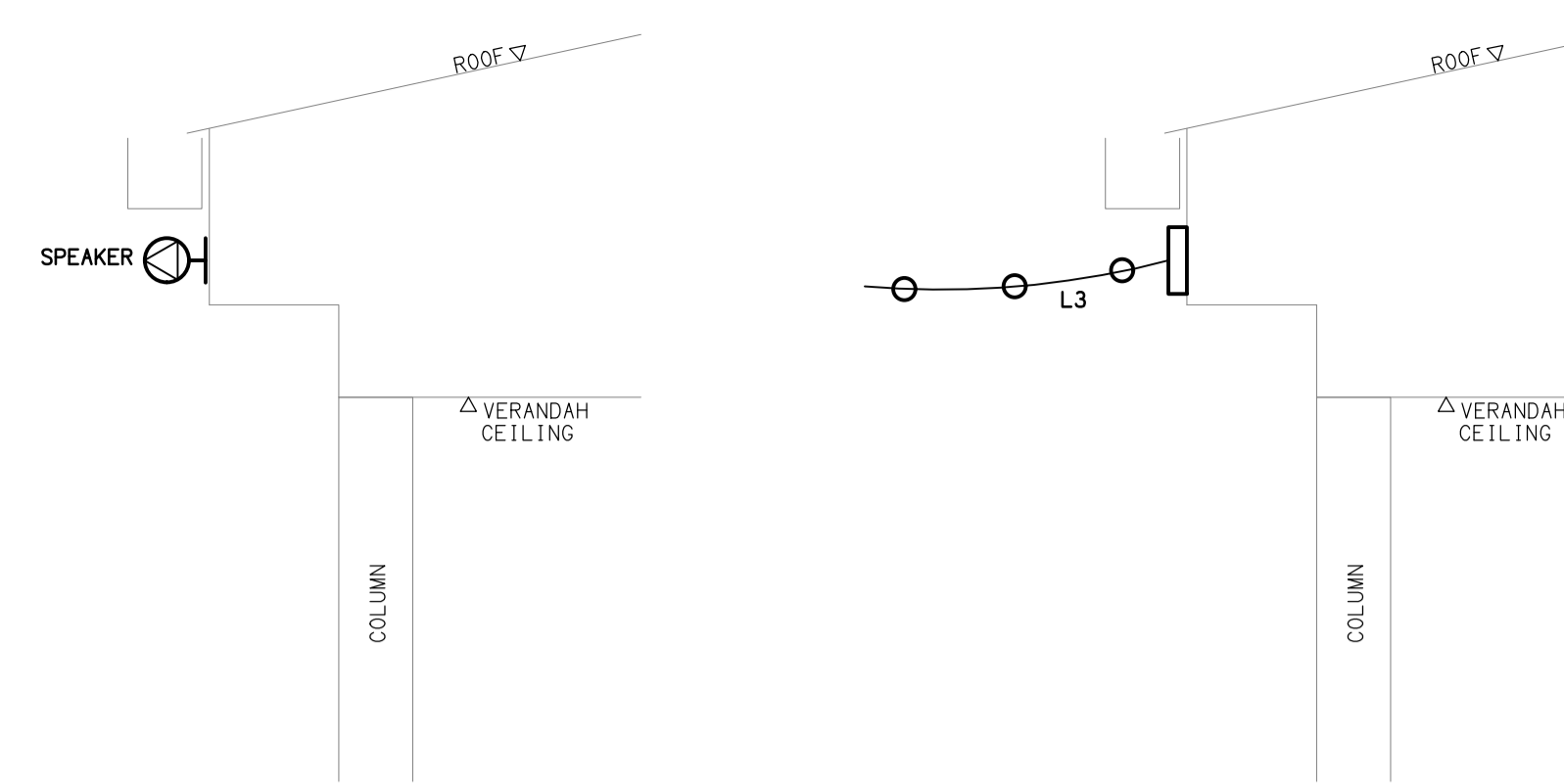
DETAIL B EXTERNAL SPEAKER MOUNTING NOT TO SCALE
