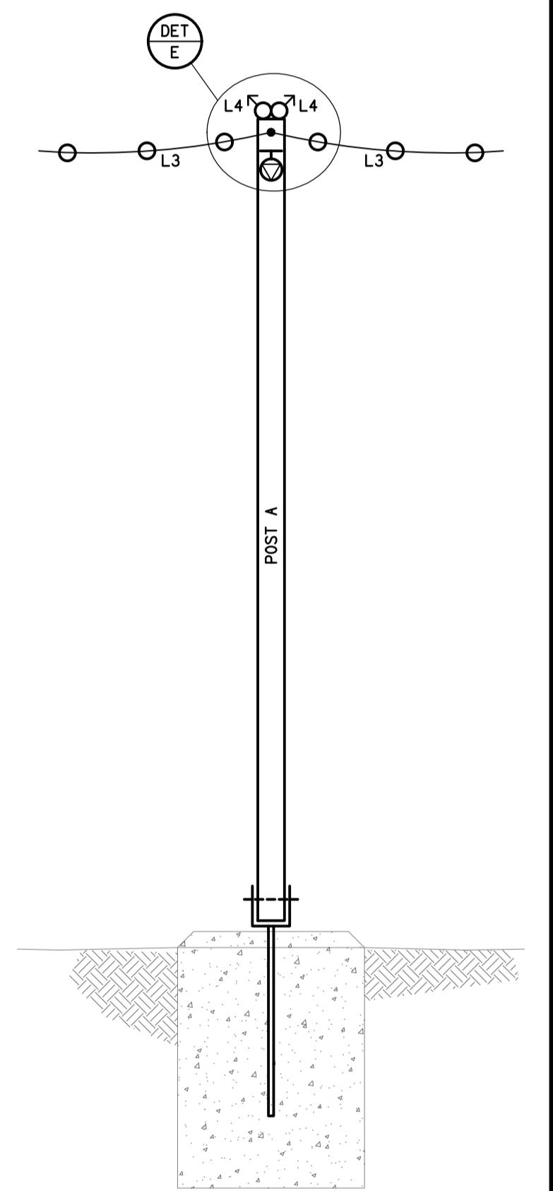
DETAIL D POST A ELEVATION NOT TO SCALE
